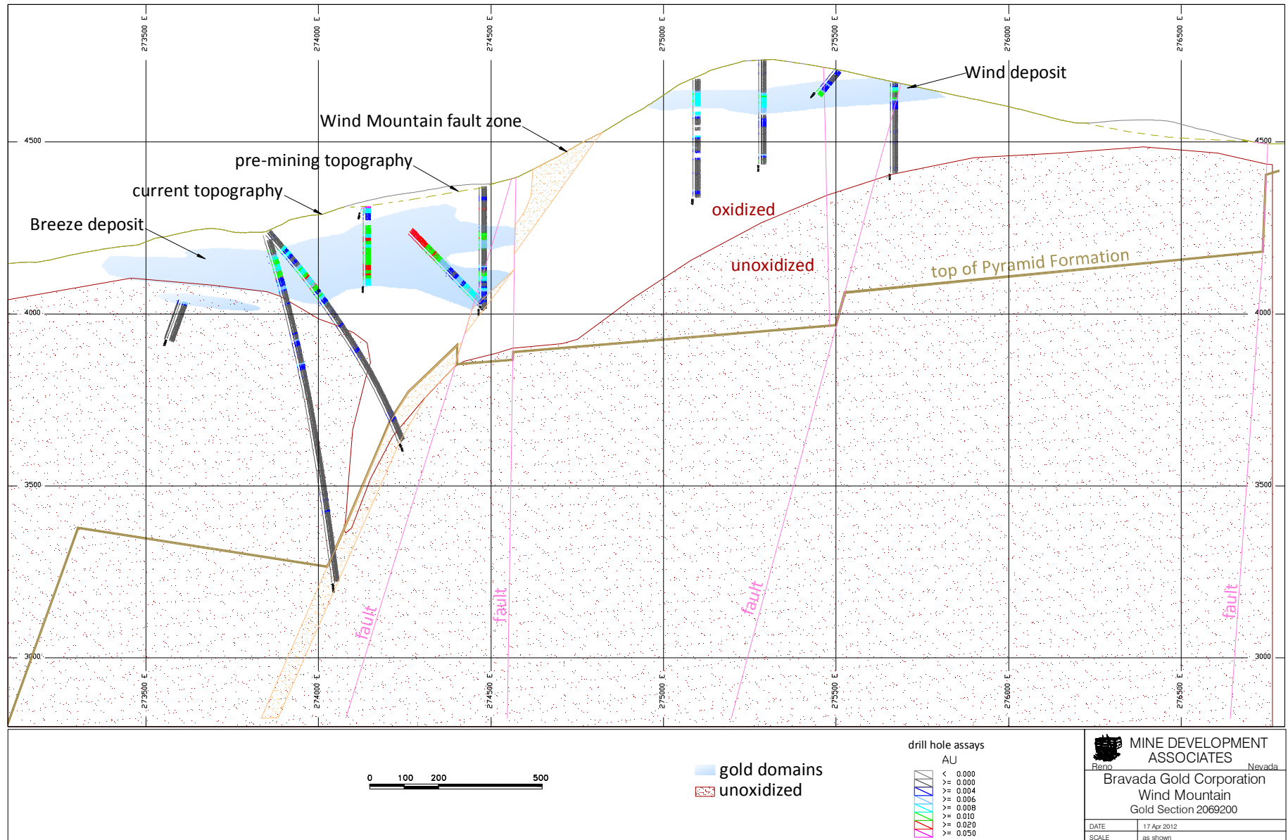
Figure 14.3 Typical Section of the Gold Mineral Domains: Wind Mountain -- Section 2069200N
