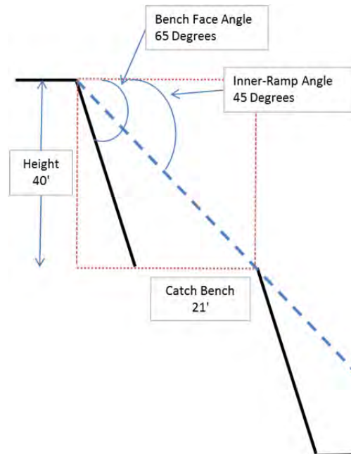
Figure 16.5 Pit Design Slope Parameters
